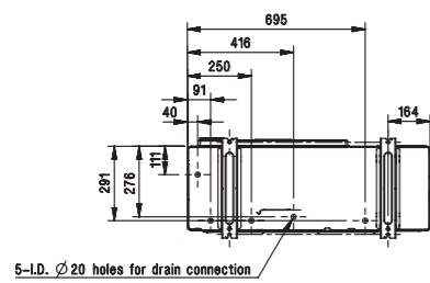
5-ID. Ø20 holes for drain connection
